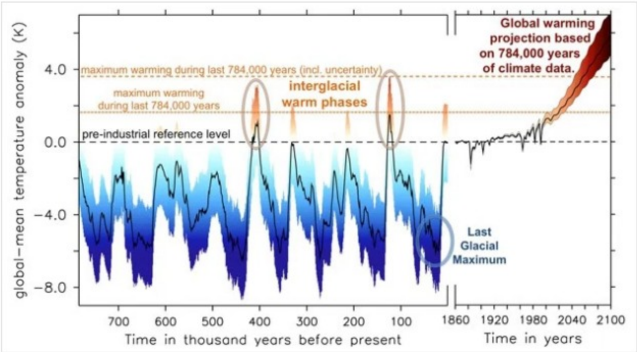
Global mean temperature anomaly with respect to preindustrial reference level.
