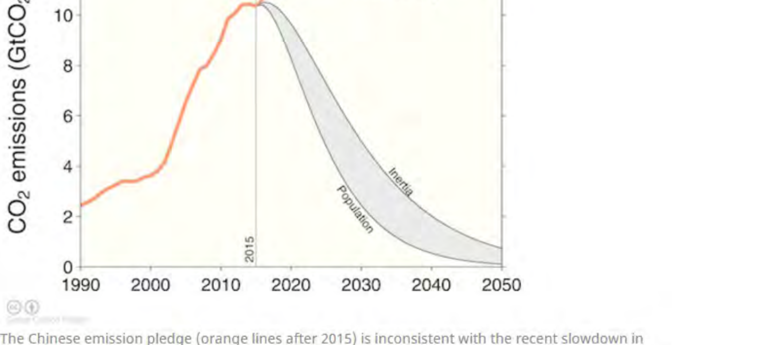
The Chinese emission pledge (orange lines after 2015) is inconsistent with the recent slowdown in emissions growth (orange lines before 2015). The grey band shows where Chinese emissions need to go to remain consistent with a 2°C temperature limit. (Source: Cicero)
