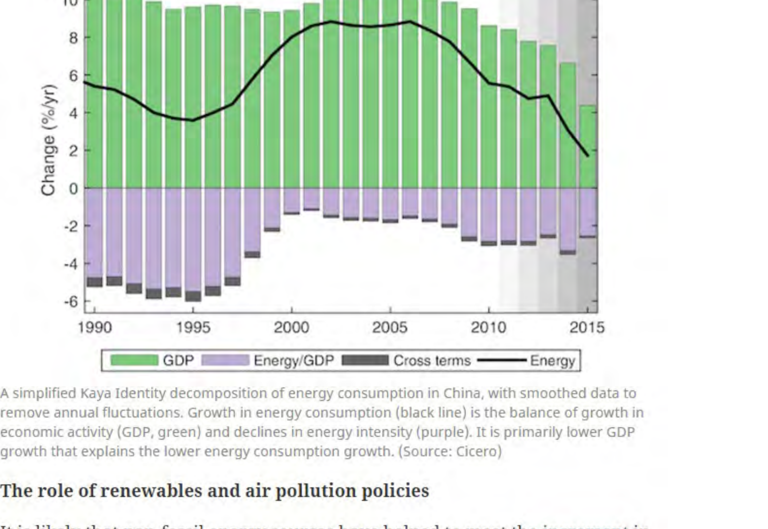
A simplified Kaya Identity decomposition of energy consumption in China, with smoothed data to remove annual fluctuations. Growth in energy consumption (black line) is the balance of growth in economic activity (GDP, green) and declines in energy intensity (purple). It is primarily lower GDP growth that explains the lower energy consumption growth. (Source: Cicero)
